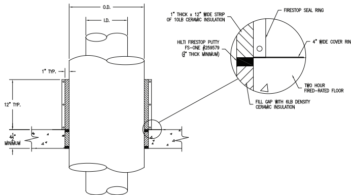
FLOOR PENETRATION
