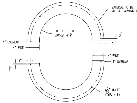
COVER RING
