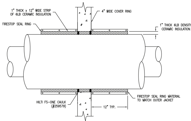
WALL PENETRATION
